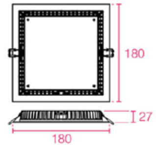
Flat 5 (15W) cross-section
