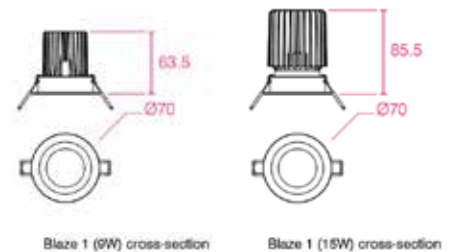
Blaze 1 (9W) cross-section
