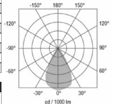
(Curve shown for 3000K with 55° beam angle) Blaze 9W polar curve.
