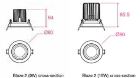
Blaze 2 (9W) cross-section
