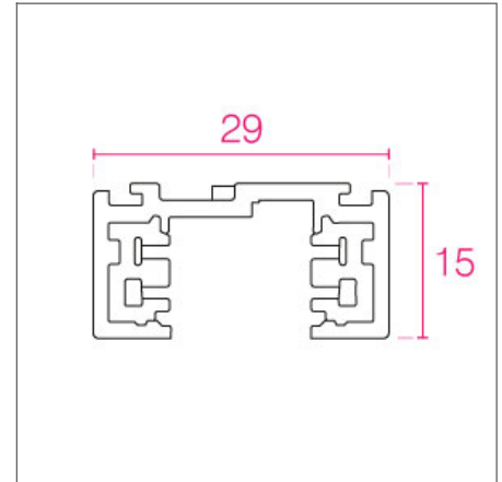
SURFACE MOUNTED PROFILE (MM)
