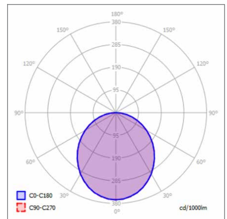
POLAR CURVE 4000K OPAL DIFFUSER
