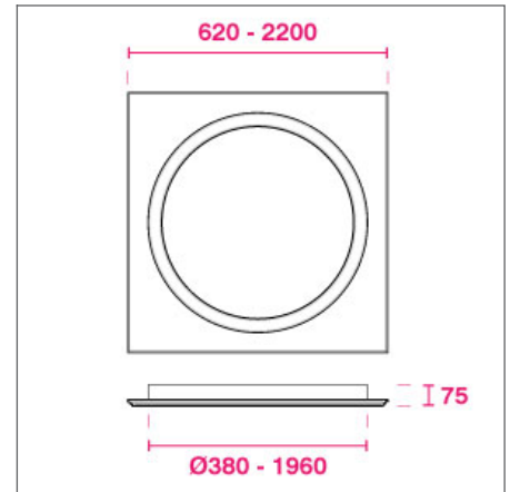
MICROBLADE CIRCLE DIMENSIONS (MM)
